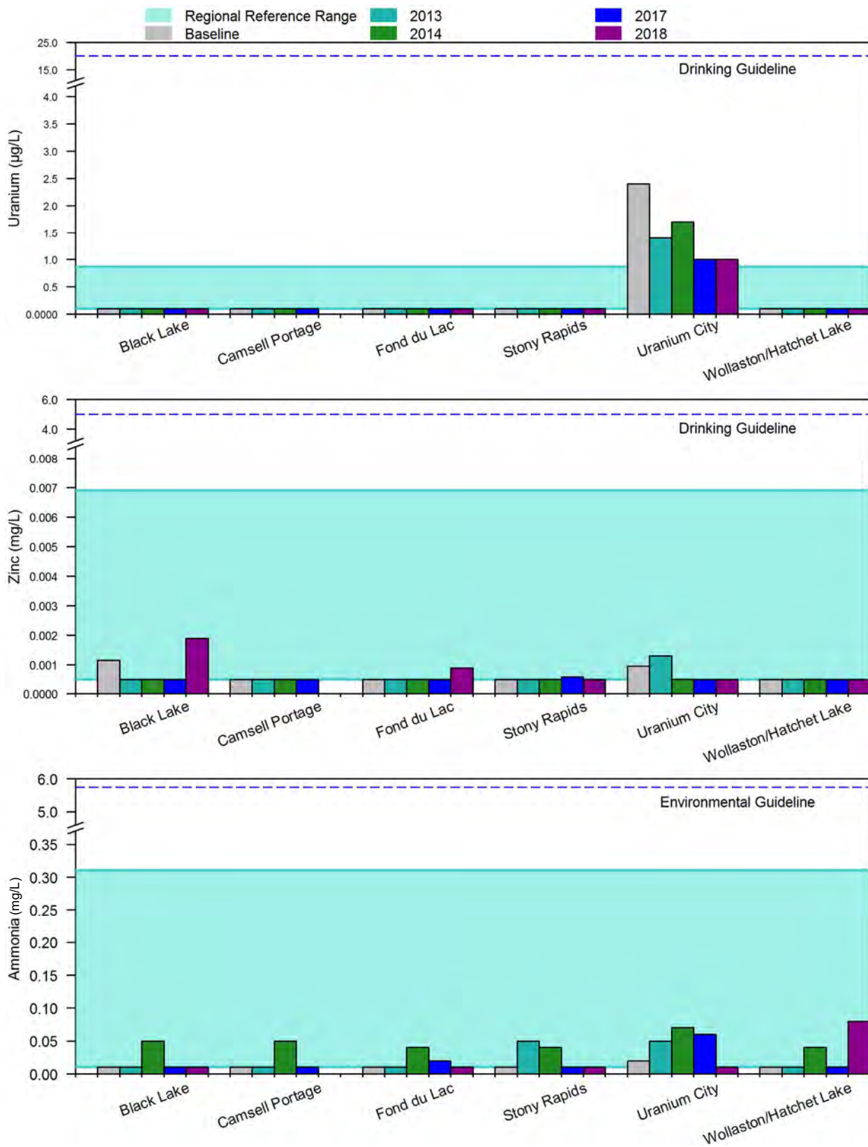
Appendix B, Figure 1 Chemicals in water from the EARMP community study area, 2011 to 2018.
